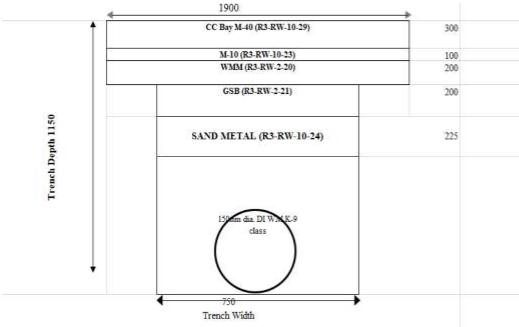
Typivcal Cross Section of Trench For Laying of 150 mm dia. DI WM in Cement Concrete
