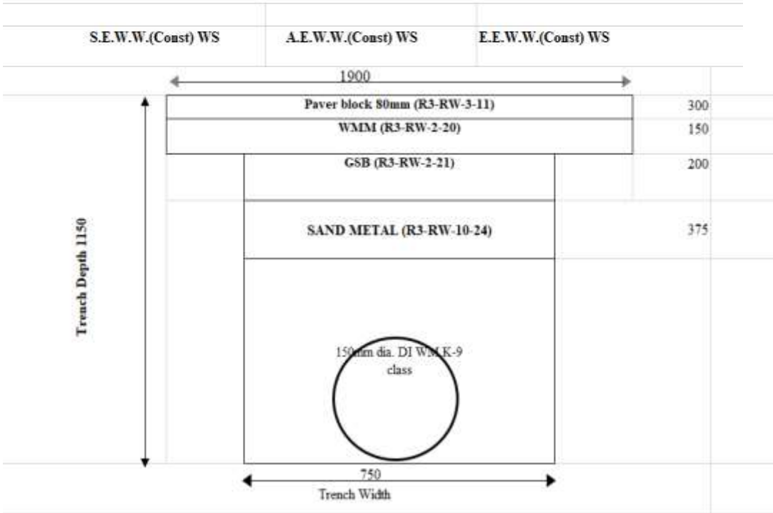
Typivcal Cross Section of Trench For Laying of 150 mm dia. DI WM in Cement Concrete
