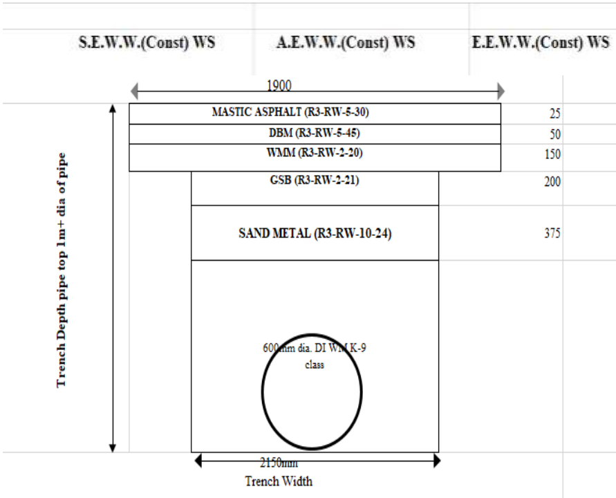
Typical Cross Section of Trench For Laying of 600mm dia. DI WM in Mastic Asphalt
